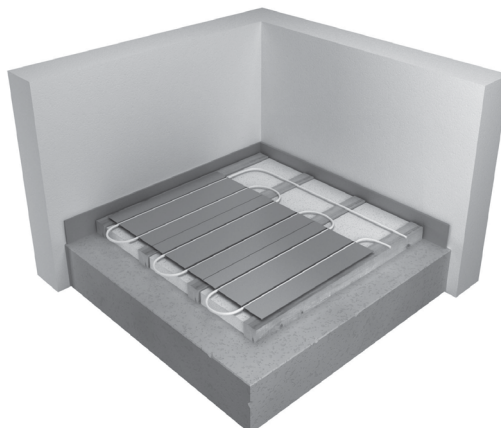
Distribute the plates evenly across the floor.
